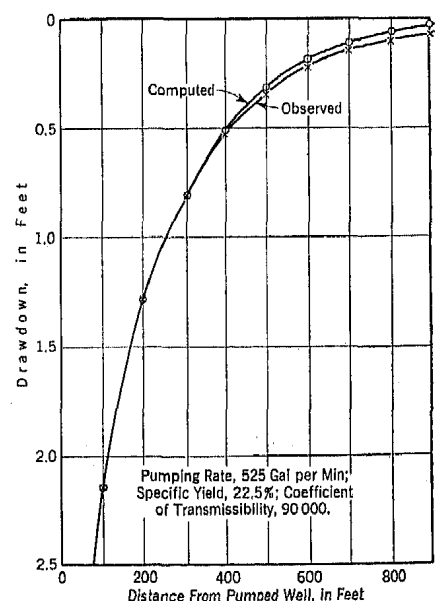
FIG. 3. OBSERVED AND COMPUTED DRAWDOWNS IN VICINITY OF A WELL AFTER PUMPING 48 HOURS
