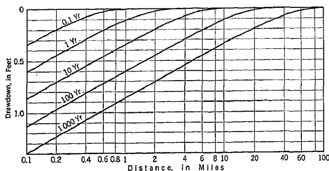
FIG. 5. DRAWDOWN FOR SAME CONDITIONS AS THOSE OF FIG. 4, PLOTTED AGAINST DISTANCE FROM DISCHARGING WELL
